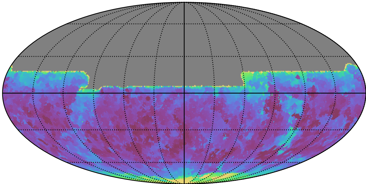
roll_pause_mjdp180_v3.4_10yrs All sky y band: Min seeingEff
