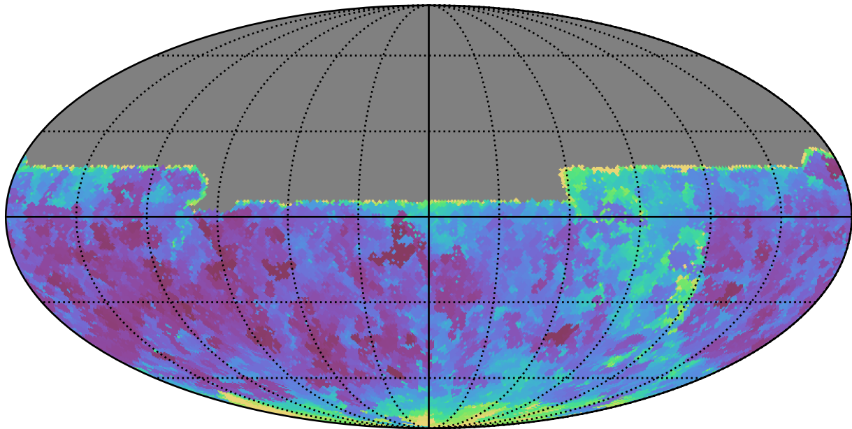
roll_pause_mjdp180_v3.4_10yrs All sky u band: Min seeingEff
