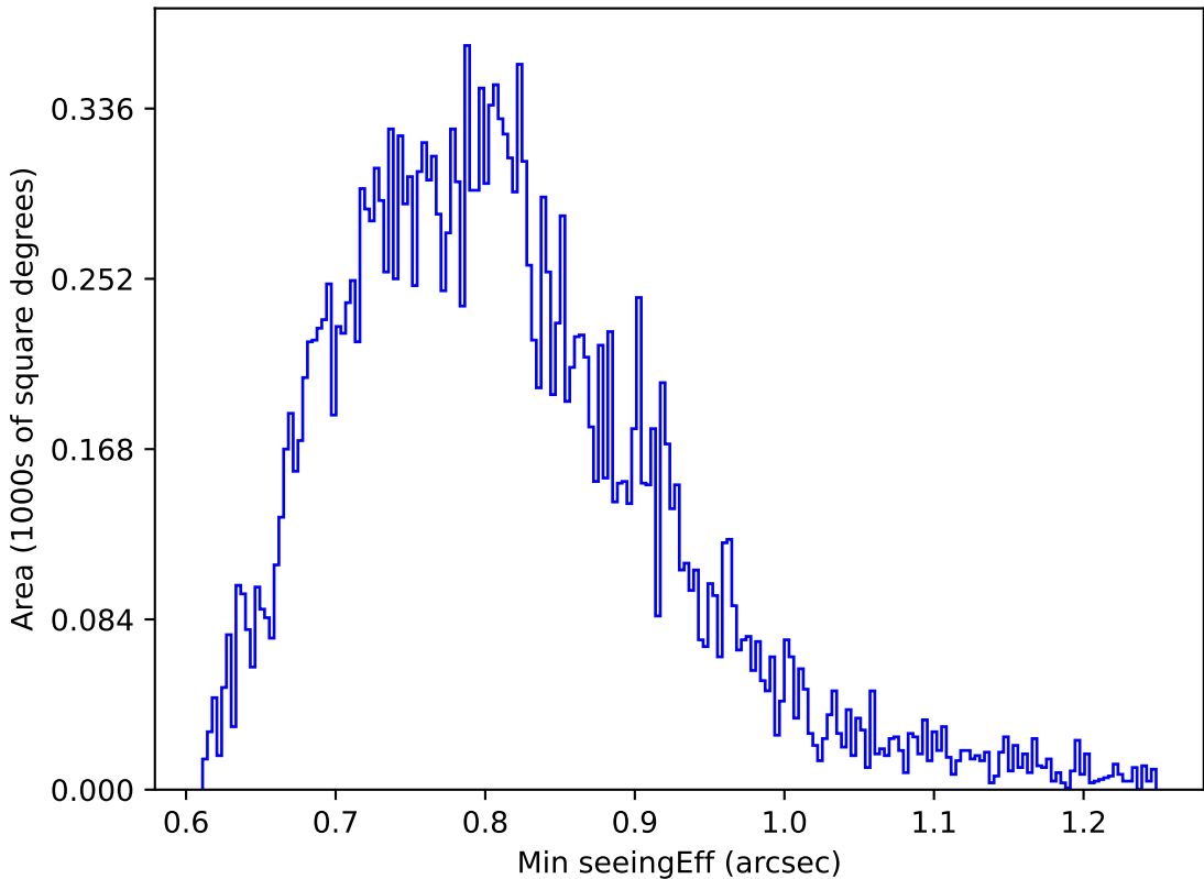
roll_pause_mjdp180_v3.4_10yrs All sky u band: Min seeingEff
