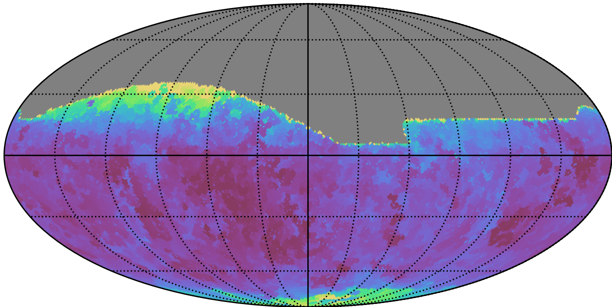
roll_pause_mjdp180_v3.4_10yrs All sky r band: Min seeingEff
