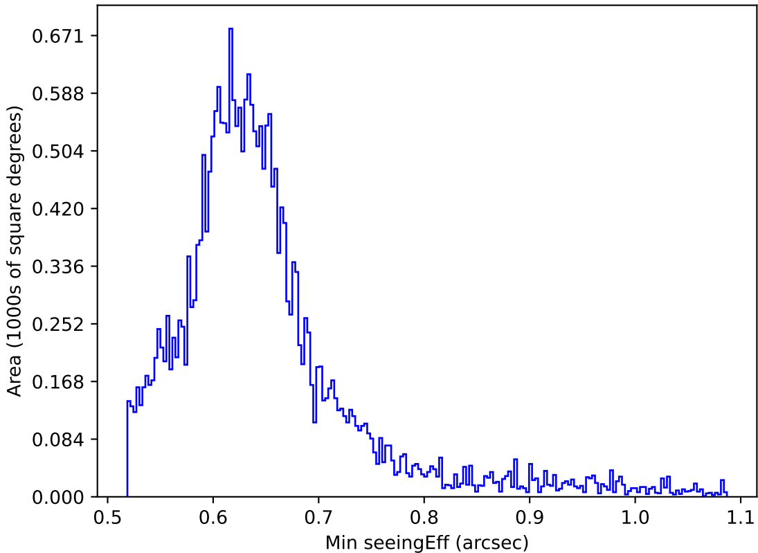
roll_pause_mjdp180_v3.4_10yrs All sky r band: Min seeingEff
