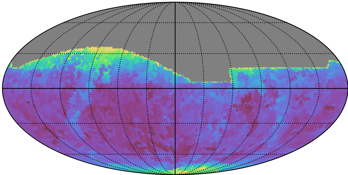
roll_pause_mjdp180_v3.4_10yrs All sky i band: Min seeingEff
