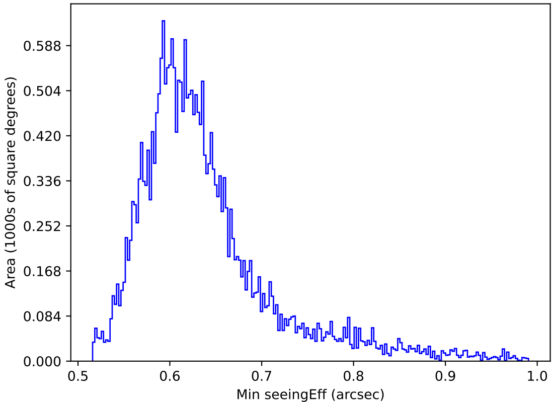
roll_pause_mjdp180_v3.4_10yrs All sky i band: Min seeingEff
