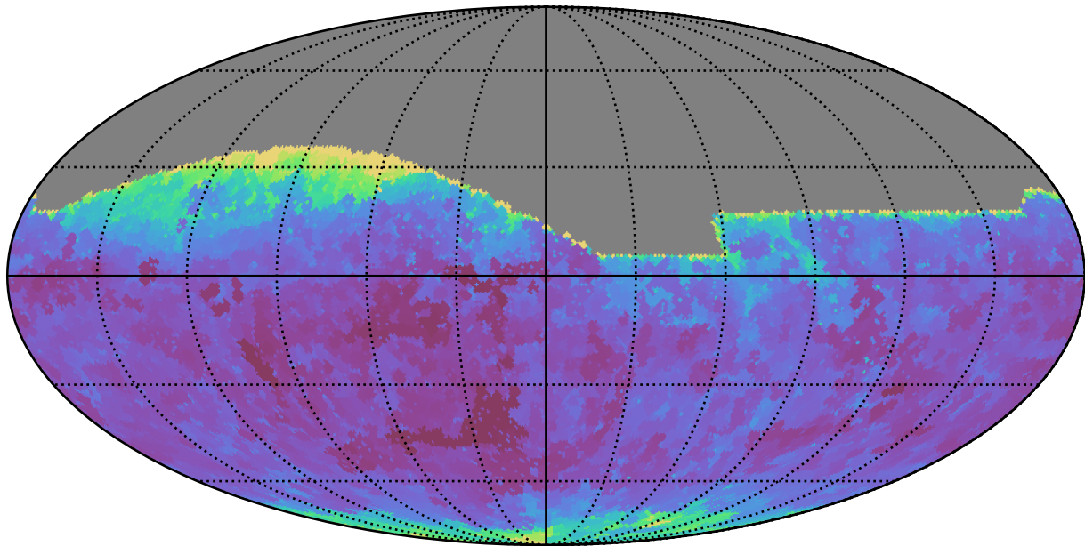
roll_pause_mjdp180_v3.4_10yrs All sky g band: Min seeingEff
