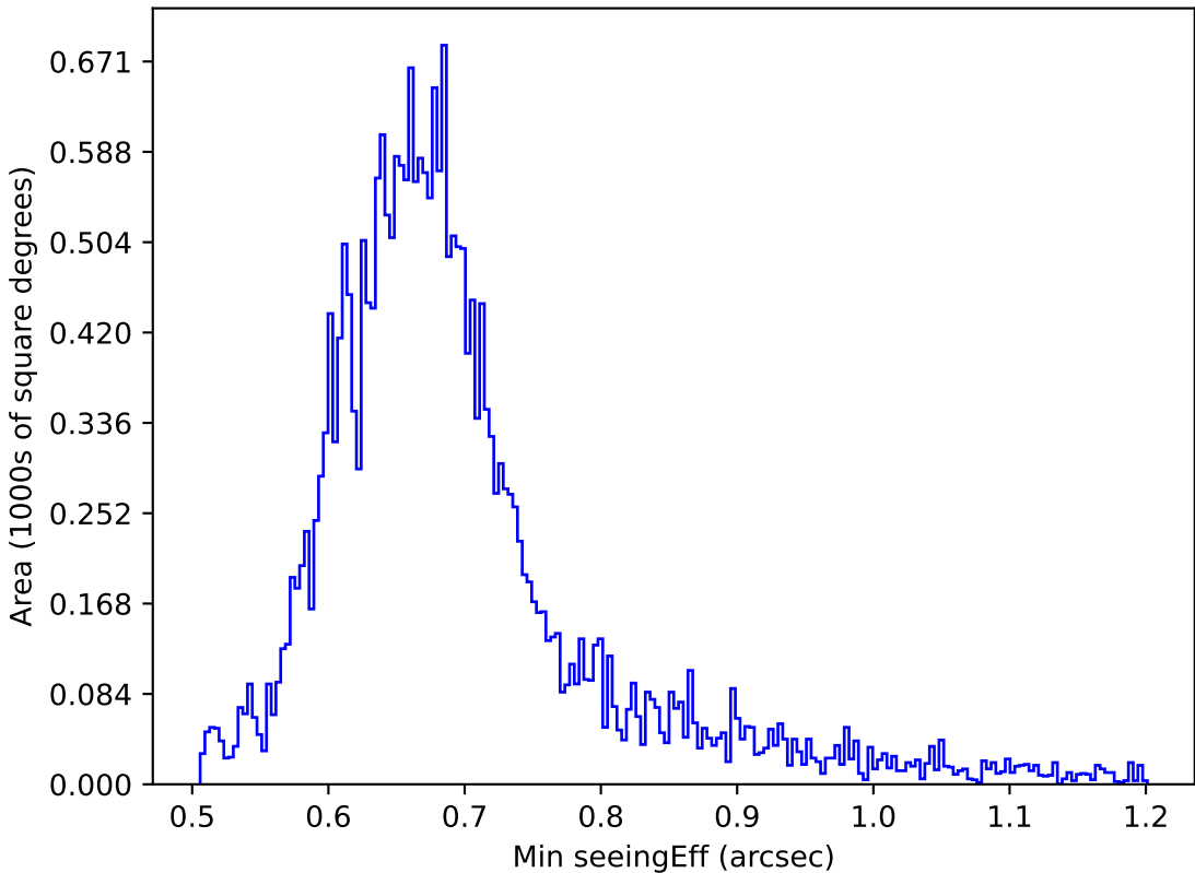
roll_pause_mjdp180_v3.4_10yrs All sky g band: Min seeingEff
