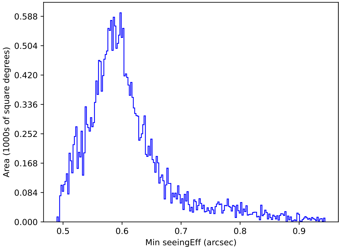
roll_pause_mjdp180_v3.4_10yrs All sky all bands: Min seeingEff
