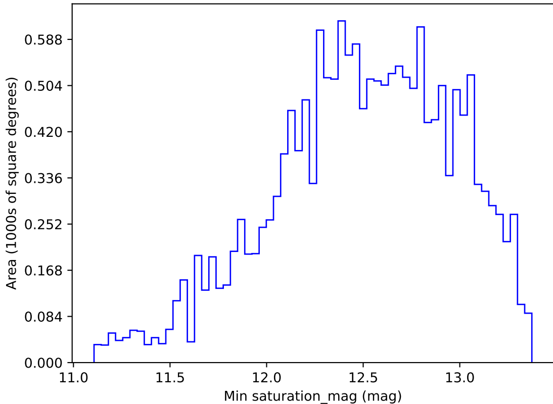
roll_pause_mjdp180_v3.4_10yrs WFD r band: Min saturation_mag
