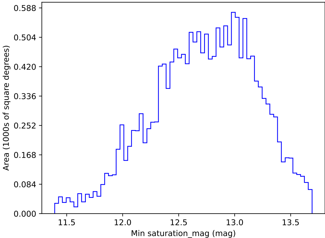
roll_pause_mjdp180_v3.4_10yrs WFD g band: Min saturation_mag
