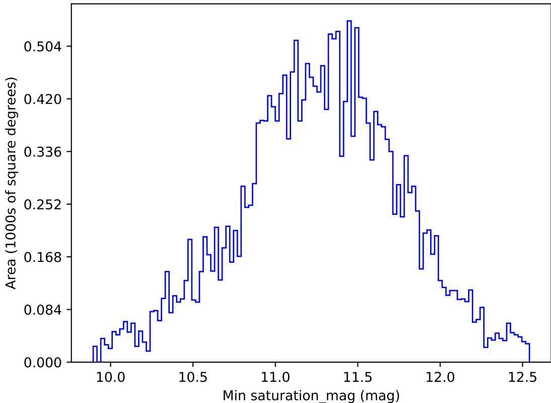
roll_pause_mjdp180_v3.4_10yrs All sky y band: Min saturation_mag
