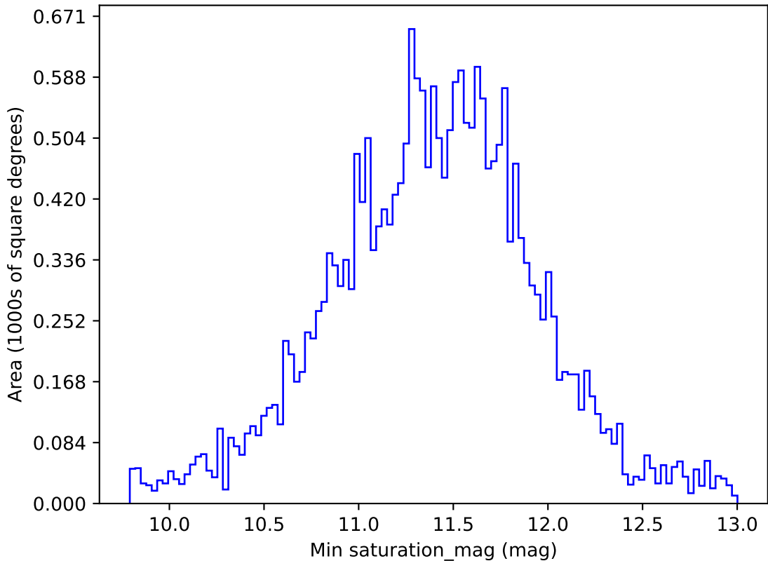
roll_pause_mjdp180_v3.4_10yrs All sky u band: Min saturation_mag
