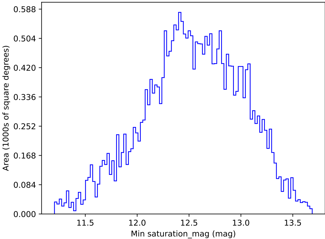
roll_pause_mjdp180_v3.4_10yrs All sky r band: Min saturation_mag
