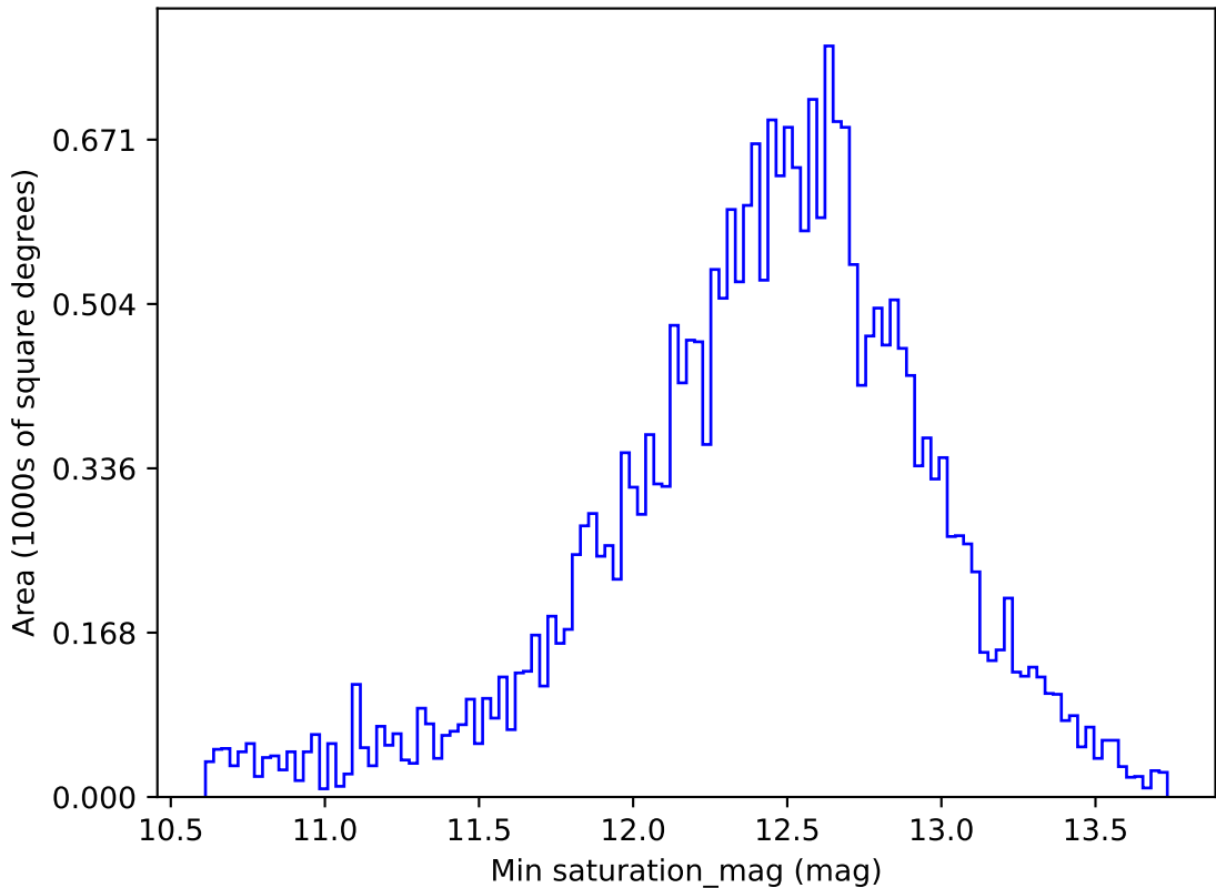
roll_pause_mjdp180_v3.4_10yrs All sky i band: Min saturation_mag
