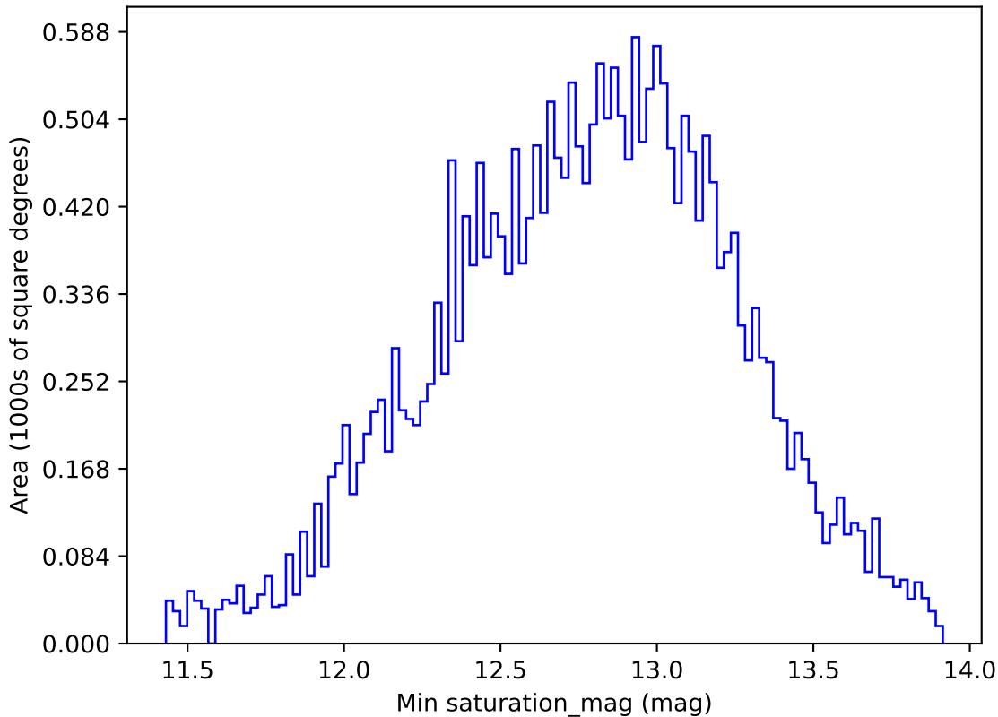
roll_pause_mjdp180_v3.4_10yrs All sky g band: Min saturation_mag
