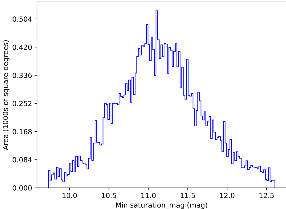
roll_pause_mjdp180_v3.4_10yrs All sky all bands: Min saturation_mag
