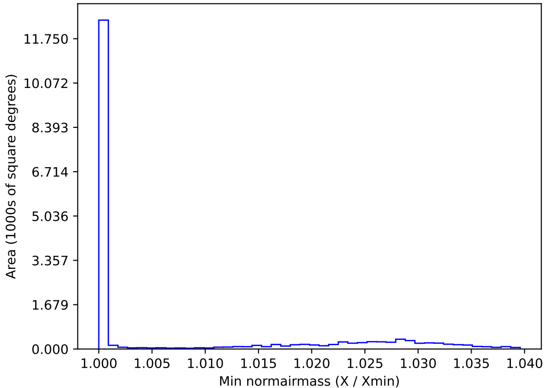
roll_pause_mjdp180_v3.4_10yrs WFD y band: Min normairmass
