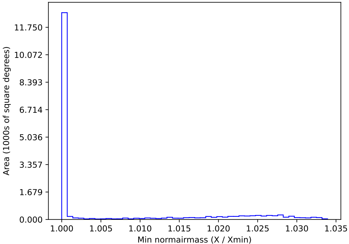
roll_pause_mjdp180_v3.4_10yrs WFD i band: Min normairmass
