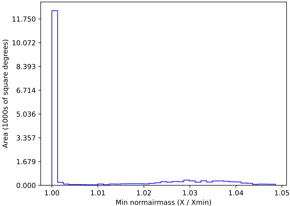
roll_pause_mjdp180_v3.4_10yrs WFD g band: Min normairmass
