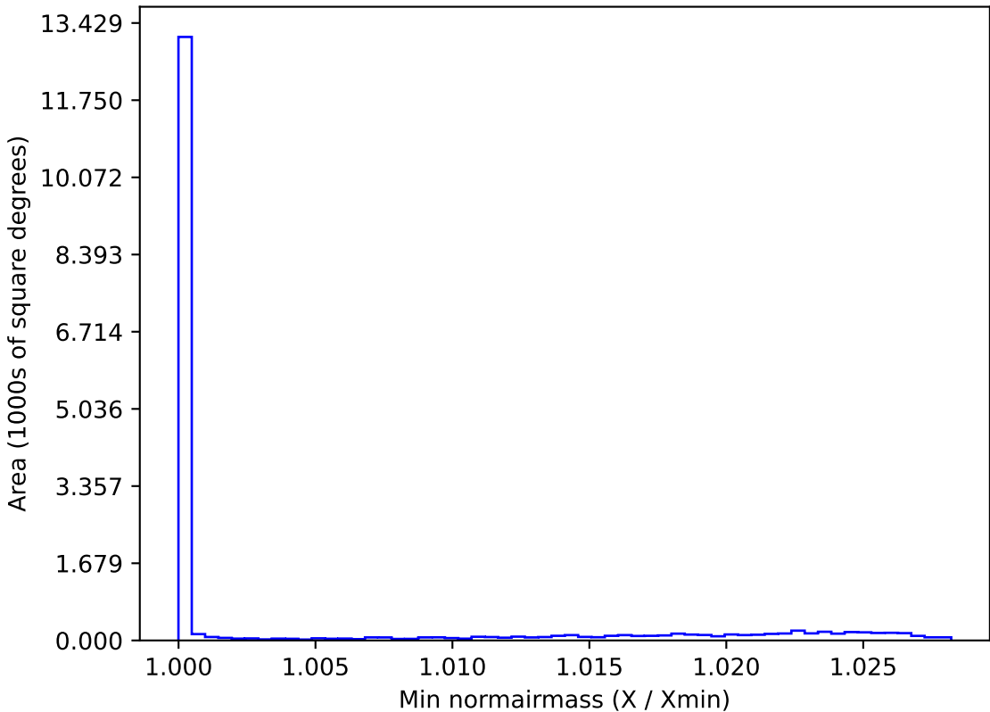
roll_pause_mjdp180_v3.4_10yrs WFD all bands: Min normairmass
