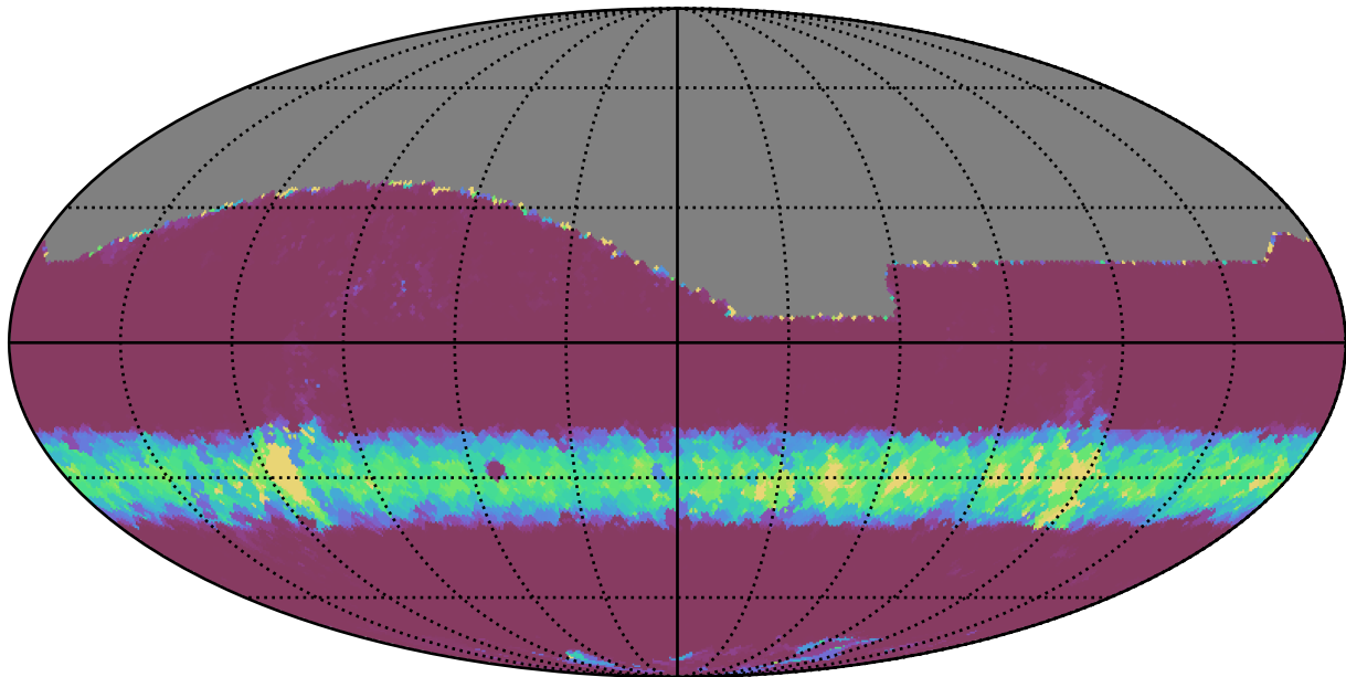
roll_pause_mjdp180_v3.4_10yrs All sky z band: Min normairmass
