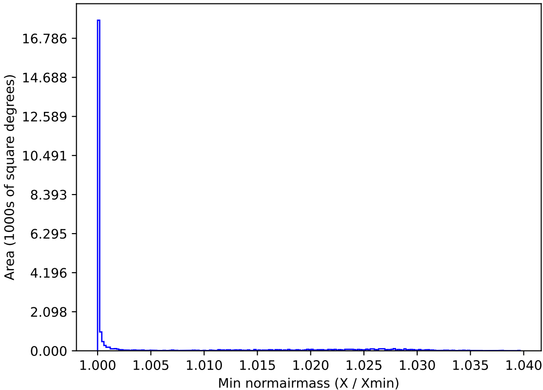
roll_pause_mjdp180_v3.4_10yrs All sky z band: Min normairmass
