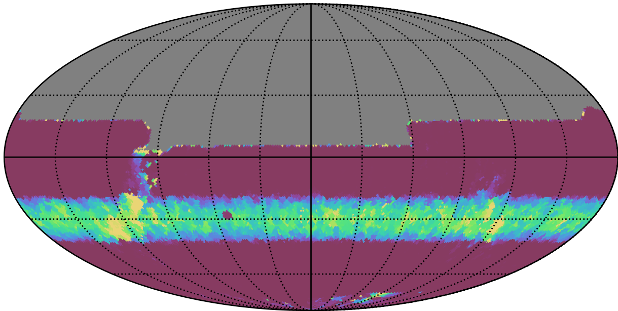
roll_pause_mjdp180_v3.4_10yrs All sky y band: Min normairmass
