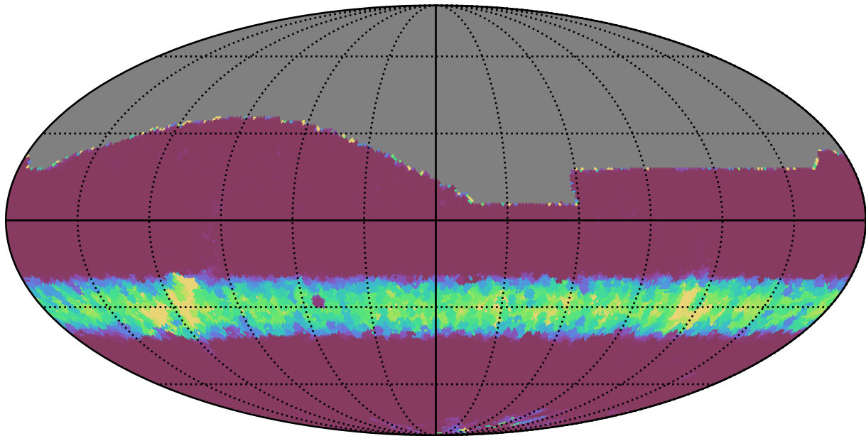
roll_pause_mjdp180_v3.4_10yrs All sky i band: Min normairmass
