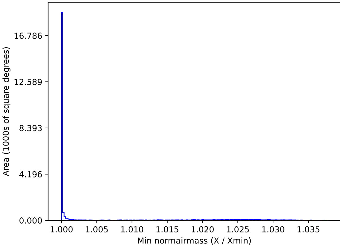
roll_pause_mjdp180_v3.4_10yrs All sky i band: Min normairmass
