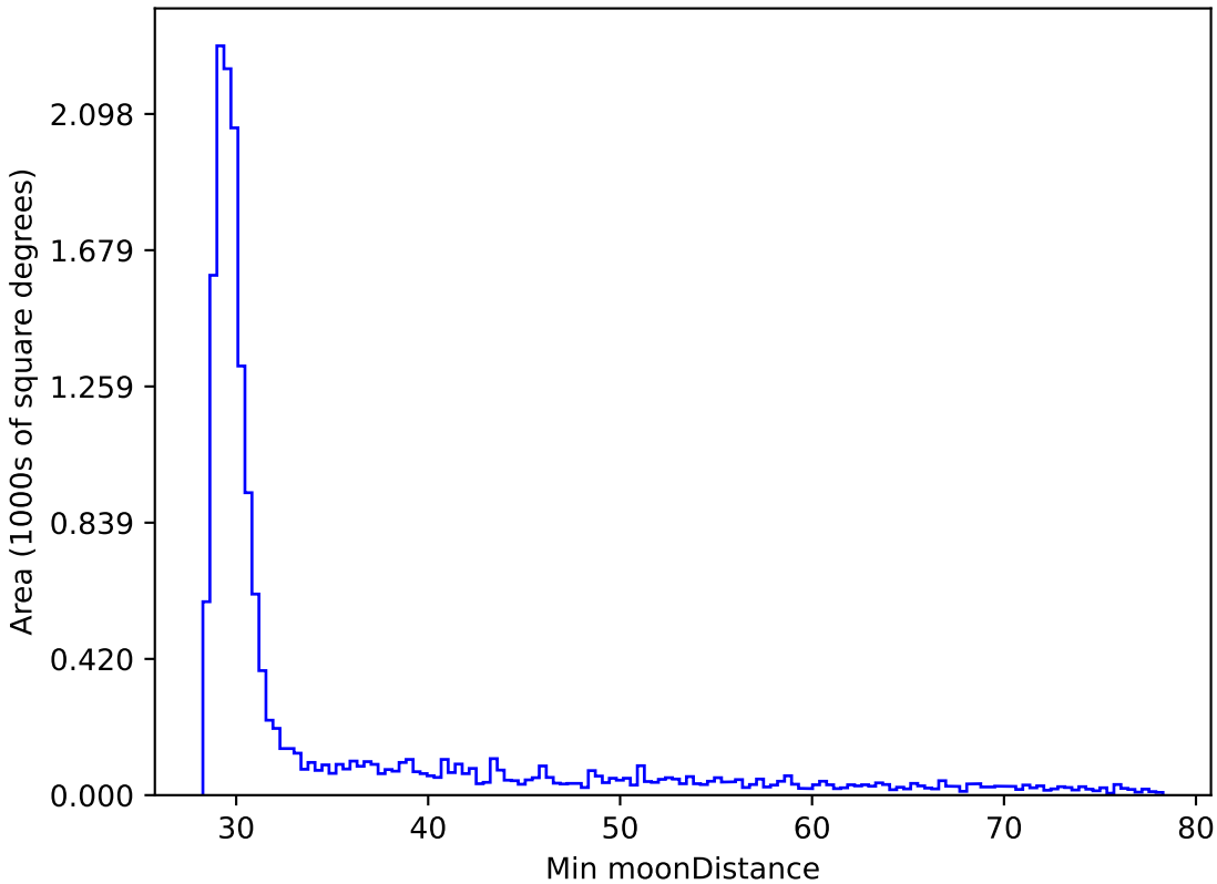
roll_pause_mjdp180_v3.4_10yrs WFD z band: Min moonDistance
