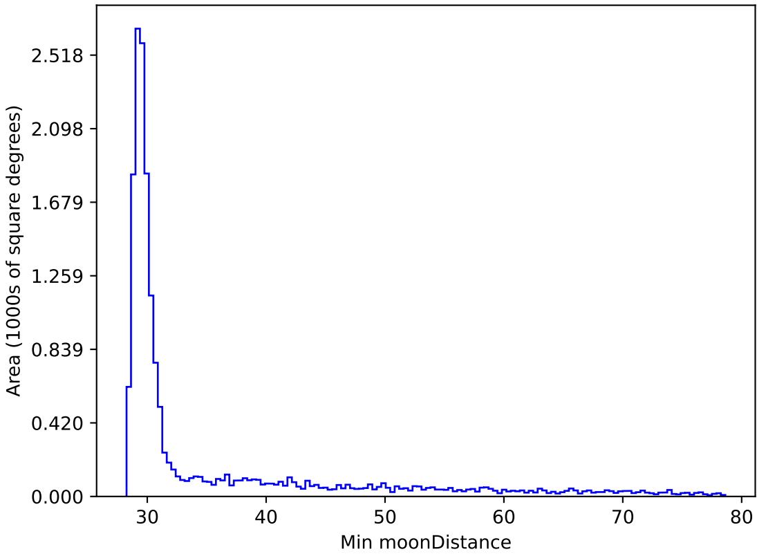
roll_pause_mjdp180_v3.4_10yrs WFD y band: Min moonDistance
