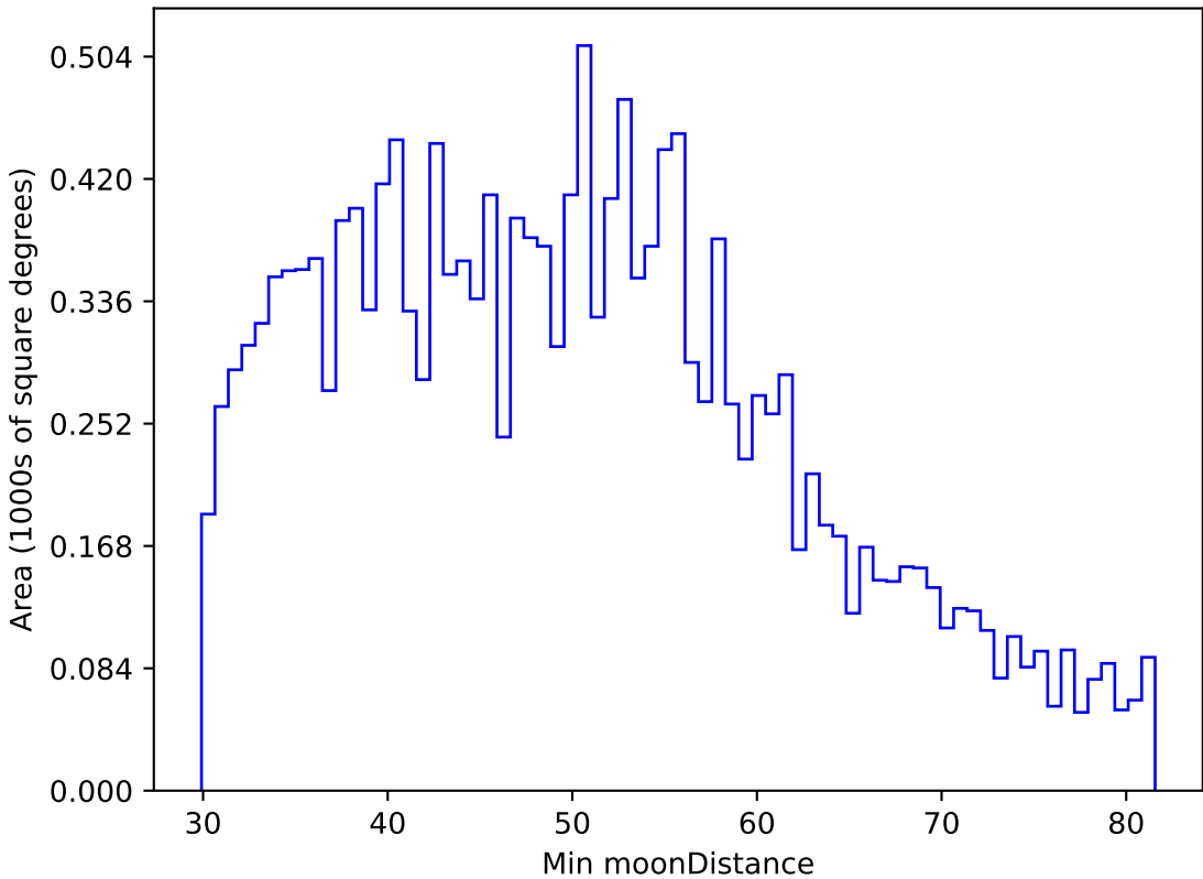
roll_pause_mjdp180_v3.4_10yrs WFD u band: Min moonDistance
