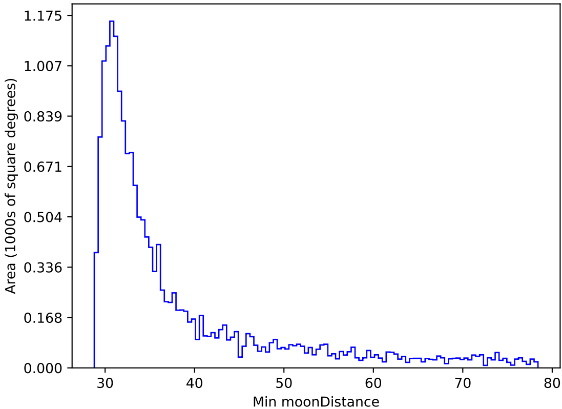
roll_pause_mjdp180_v3.4_10yrs WFD r band: Min moonDistance
