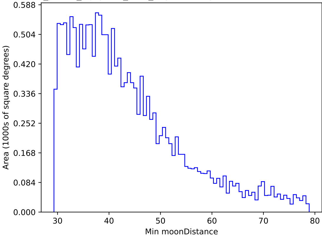
roll_pause_mjdp180_v3.4_10yrs WFD g band: Min moonDistance
