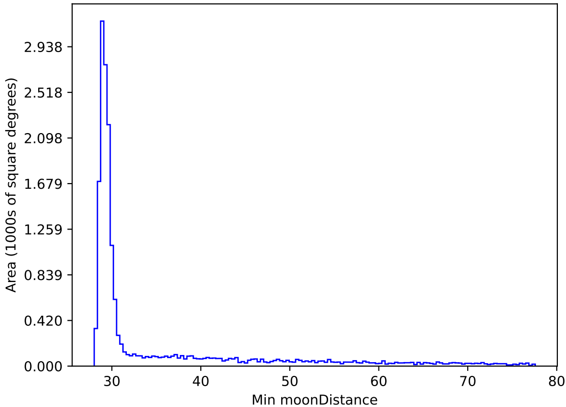
roll_pause_mjdp180_v3.4_10yrs WFD all bands: Min moonDistance
