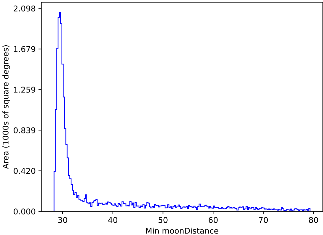
roll_pause_mjdp180_v3.4_10yrs All sky y band: Min moonDistance
