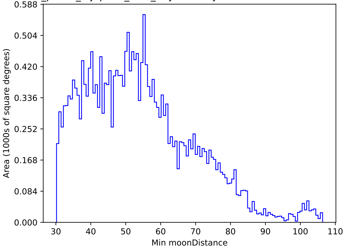
roll_pause_mjdp180_v3.4_10yrs All sky u band: Min moonDistance
