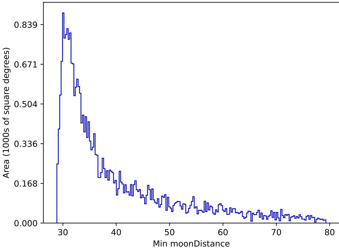
roll_pause_mjdp180_v3.4_10yrs All sky r band: Min moonDistance
