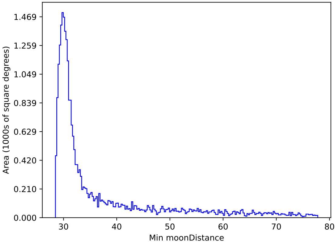
roll_pause_mjdp180_v3.4_10yrs All sky i band: Min moonDistance
