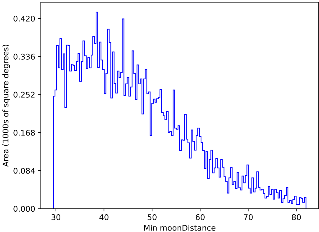
roll_pause_mjdp180_v3.4_10yrs All sky g band: Min moonDistance
