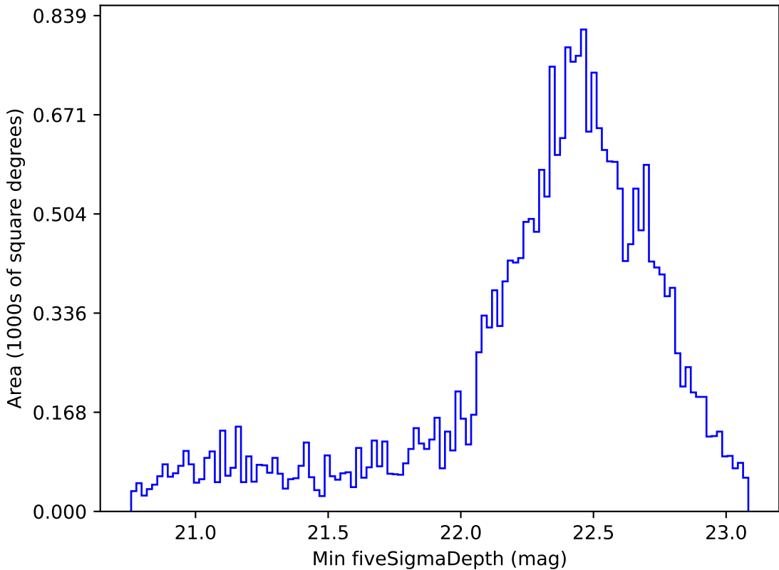
roll_pause_mjdp180_v3.4_10yrs Yr 1 z band: Min fiveSigmaDepth
