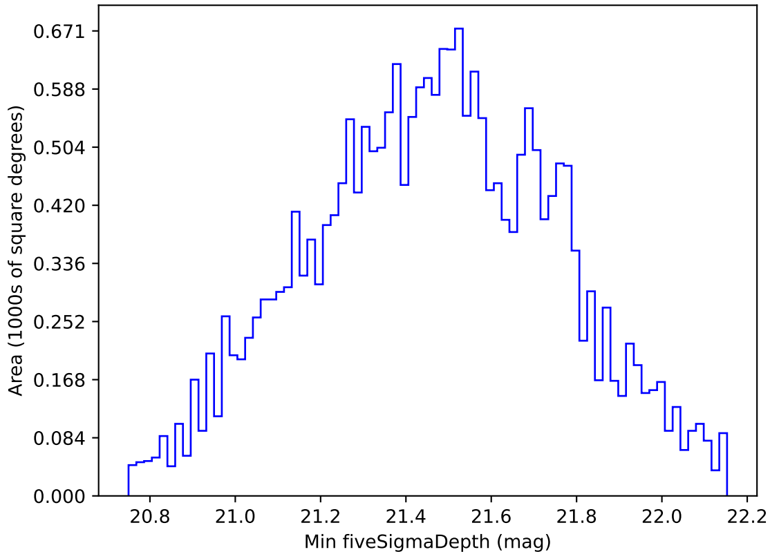
roll_pause_mjdp180_v3.4_10yrs Yr 1 y band: Min fiveSigmaDepth
