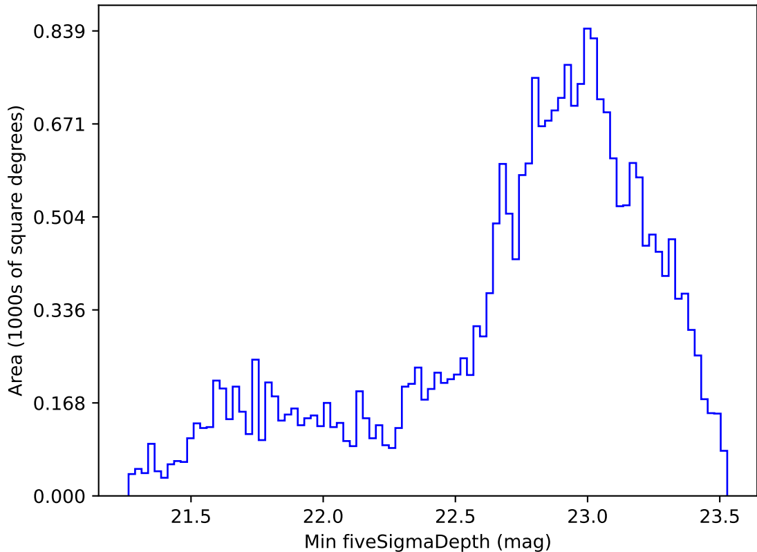
roll_pause_mjdp180_v3.4_10yrs Yr 1 i band: Min fiveSigmaDepth
