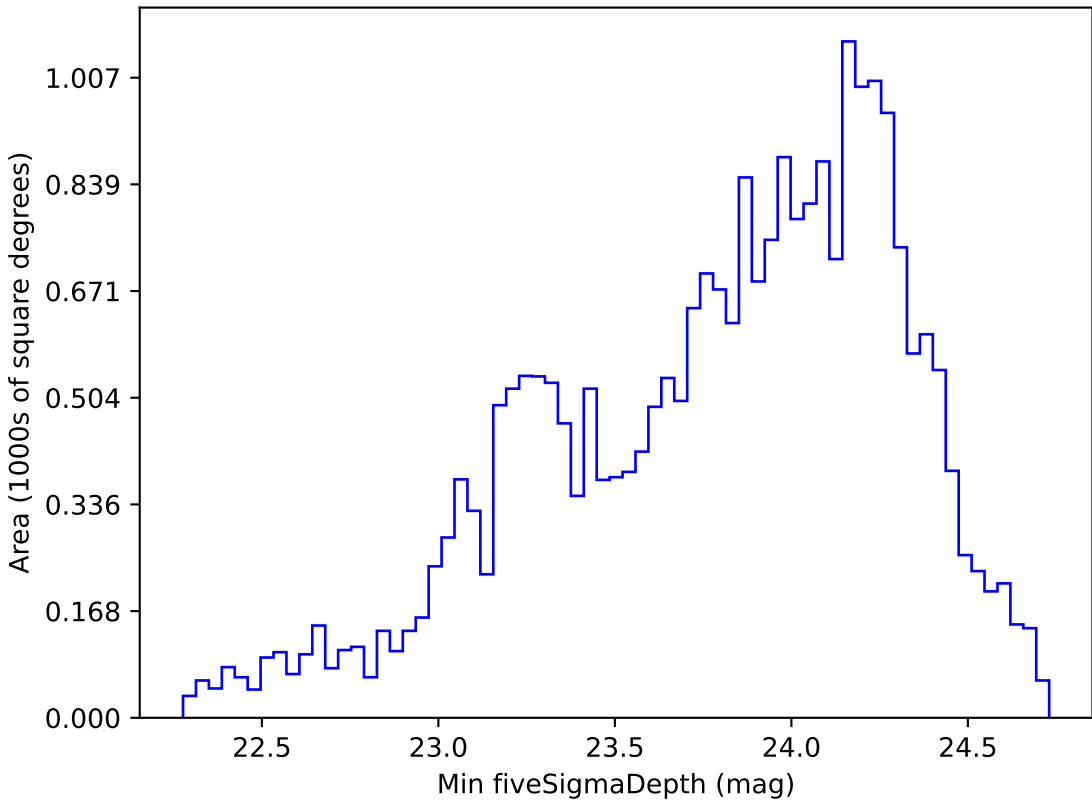
roll_pause_mjdp180_v3.4_10yrs Yr 1 g band: Min fiveSigmaDepth
