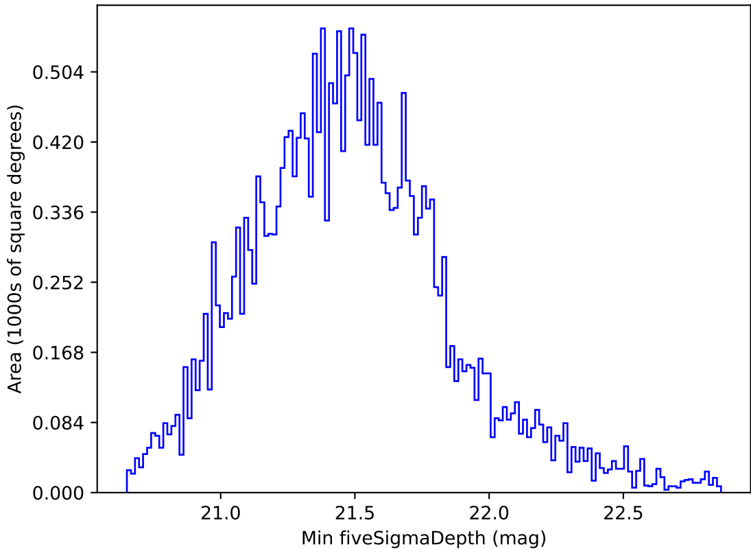
roll_pause_mjdp180_v3.4_10yrs Yr 1 all bands: Min fiveSigmaDepth
