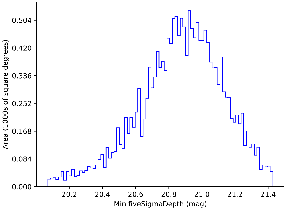
roll_pause_mjdp180_v3.4_10yrs WFD y band: Min fiveSigmaDepth
