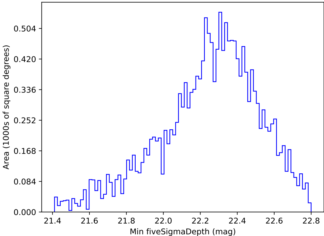
roll_pause_mjdp180_v3.4_10yrs WFD u band: Min fiveSigmaDepth
