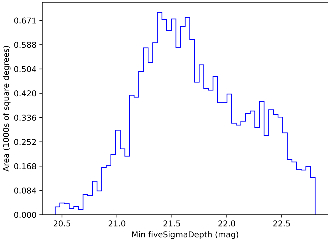
roll_pause_mjdp180_v3.4_10yrs WFD i band: Min fiveSigmaDepth
