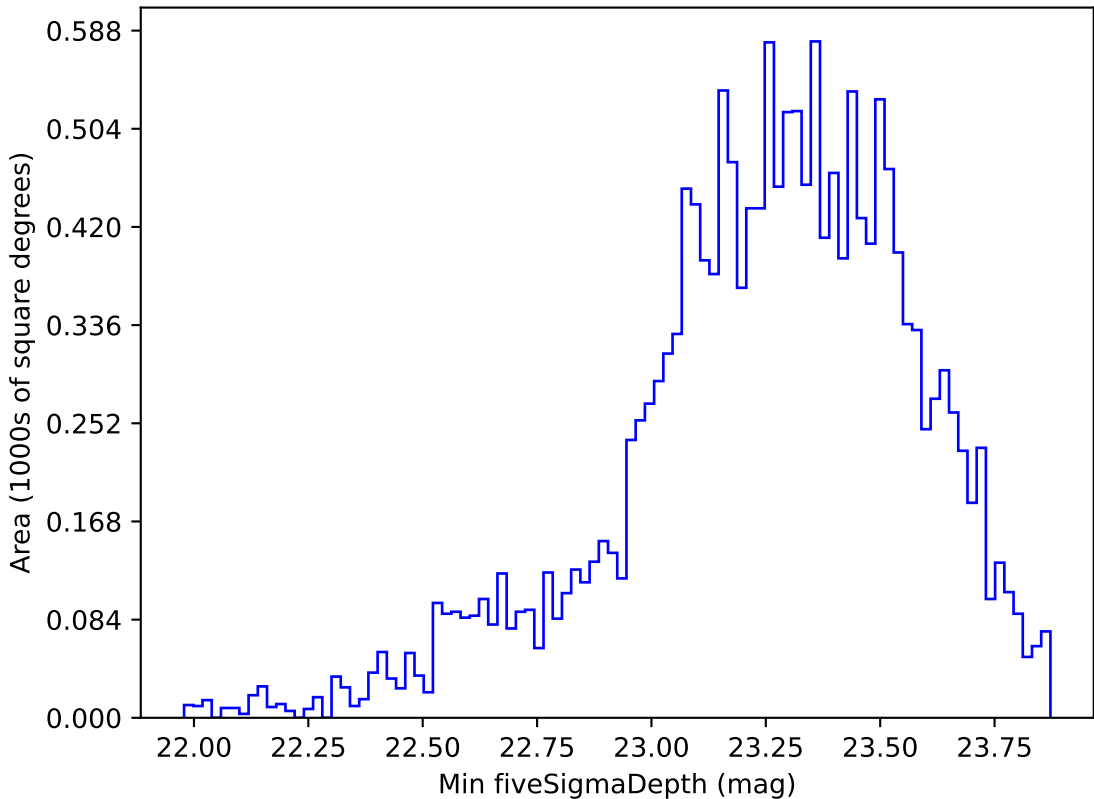
roll_pause_mjdp180_v3.4_10yrs WFD g band: Min fiveSigmaDepth
