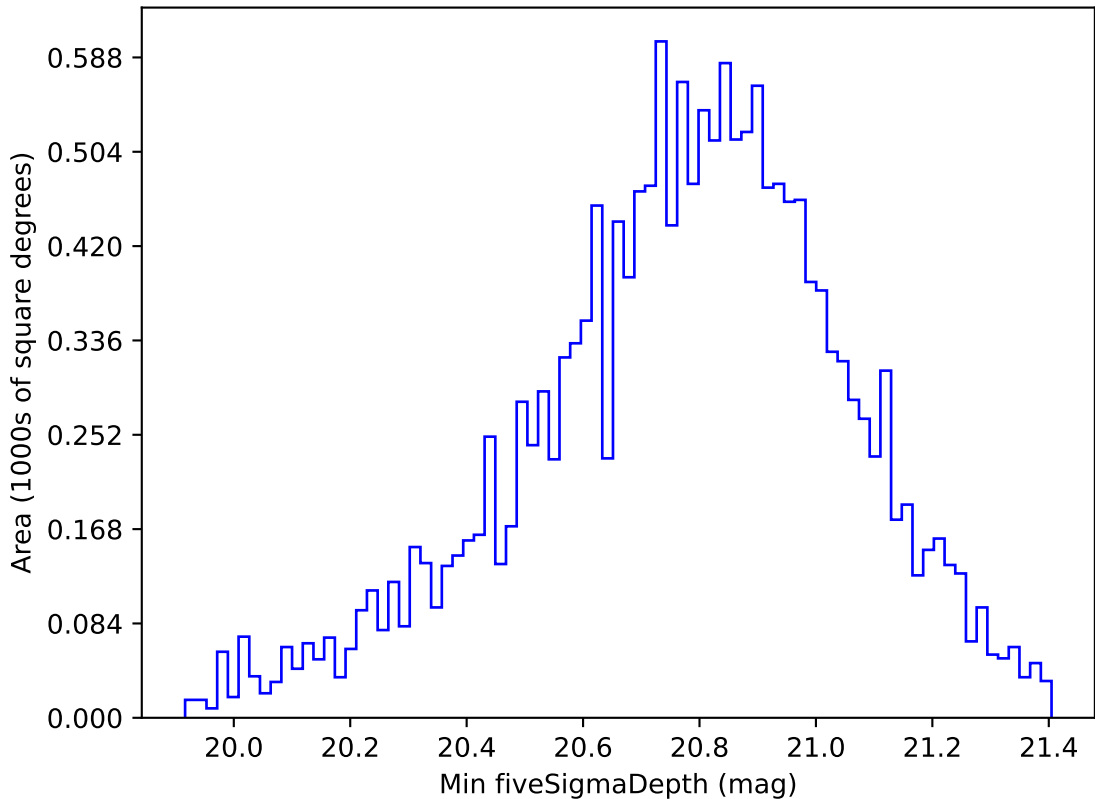
roll_pause_mjdp180_v3.4_10yrs WFD all bands: Min fiveSigmaDepth
