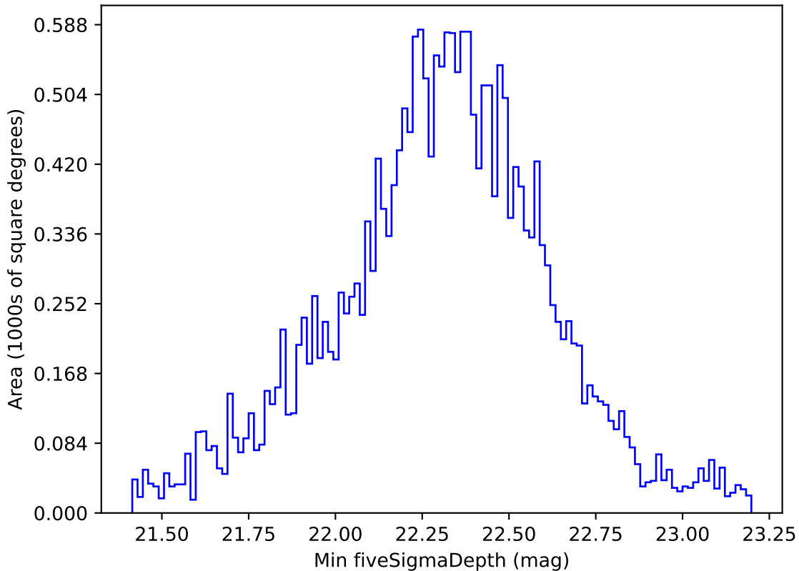
roll_pause_mjdp180_v3.4_10yrs All sky u band: Min fiveSigmaDepth
