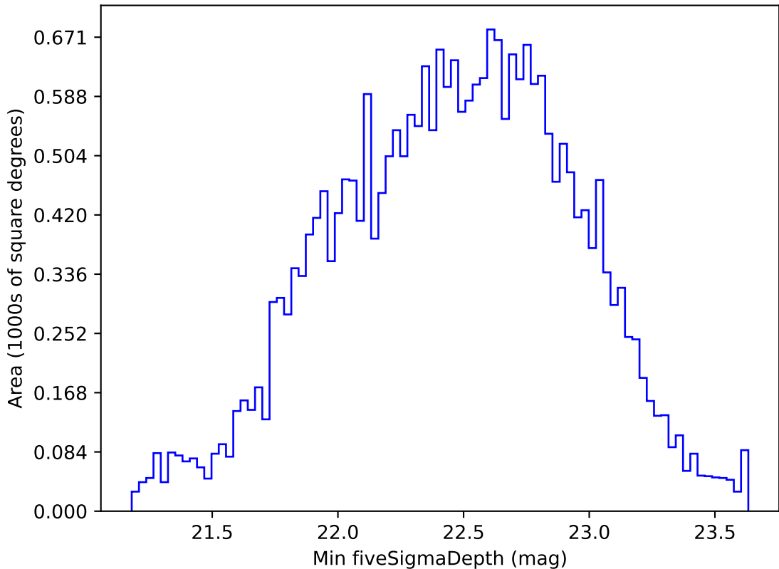
roll_pause_mjdp180_v3.4_10yrs All sky r band: Min fiveSigmaDepth
